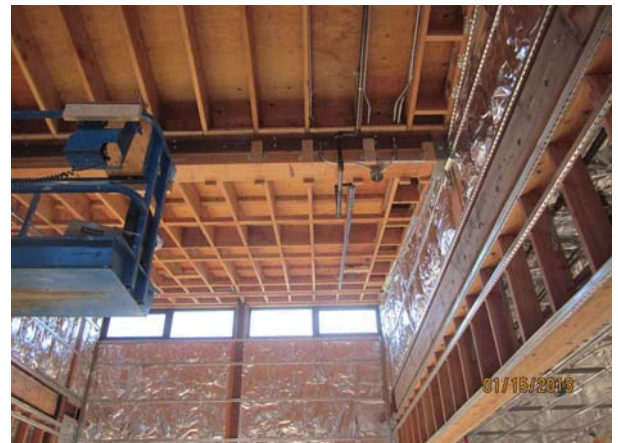
PG&E Joint Trench for Gas & Power
